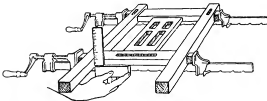
FIG. 415. TESTING POST FOR SQUARENESS TO RAIL.
